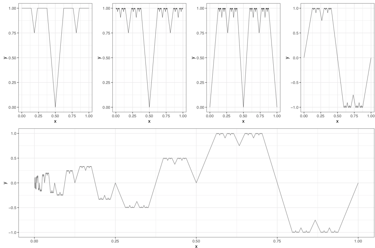
FIGURE 2. The construction used in the proof of Theorem 2.10 for the case \beta = \frac{3}{8} . The first row depicts the construction of the function f , the lower panel the function \Phi_f(\mathbf{s}) for \mathbf{s} = (s_1, s_2, s_3, \dots) with s_i = \frac{1}{i}(-1)^{i+1} .
