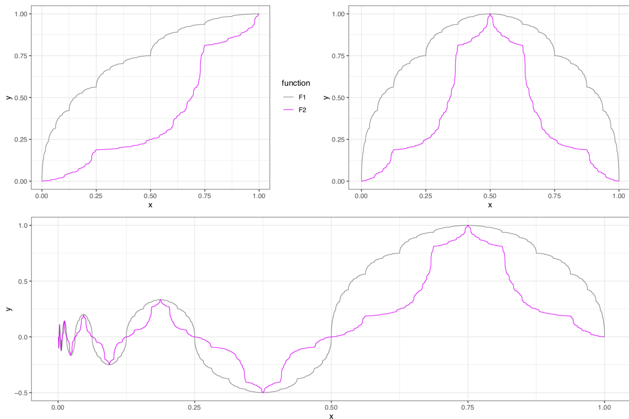
FIGURE 1. Two choices for the singular function F (upper left panel), the functions f according to equation 2.2 (upper right panel), and the resulting functions \Phi_f(\mathbf{s}) for \mathbf{s} = (s_1, s_2, s_3, \dots) with s_i = \frac{1}{2}(-1)^{i+1} (lower panel). Both functions F were constructed via fractal interpolation as discussed in [26] (see, also, [13]).
